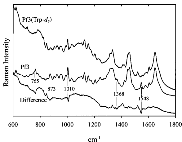
FIGURE 2 Raman spectra (600–1800 \text{cm}^{-1} , 514.5-nm excitation) of solutions of unlabeled Pf3 virus (middle trace) and labeled Pf3 virus containing deuteriotryptophan (Trp- d_5 ) at subunit residue 38 (top trace). The normalized difference spectrum is also shown (bottom trace). Samples were prepared at \sim 100 mg/mL in 10 mM Tris at pH 7.8 and data were collected at 20°C.
